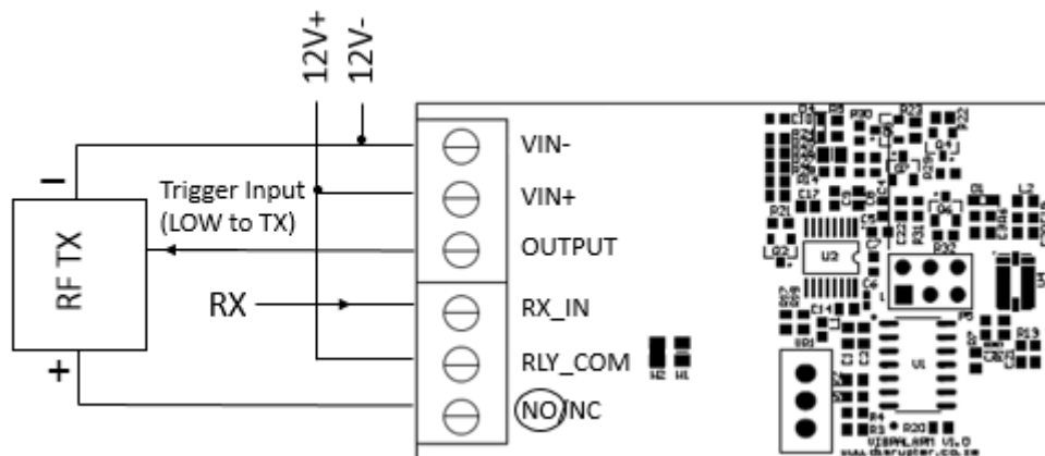
Figure 3 - Low-power connection of RF Transmitter only
